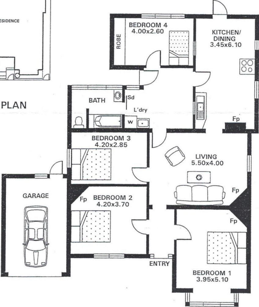
FLOOR PLAN
